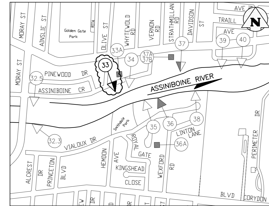
OLIVE ST. OUTFALL (AS-33)
